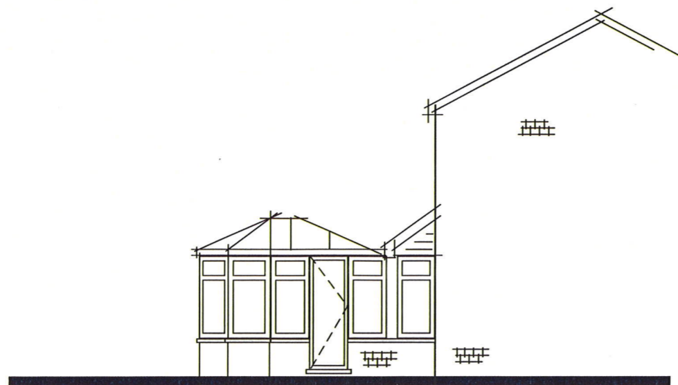
EXISTING SIDE ELEVATION (EAST)
